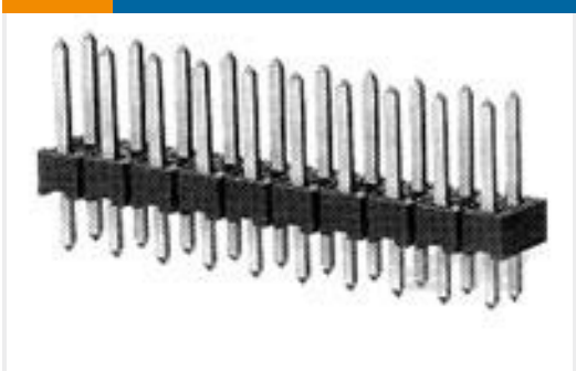
TE 产品编号1-826632-6 16P AMPMODU II STIFT LEI
