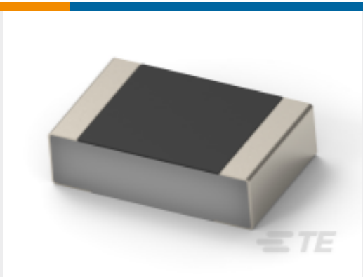
TE 产品编号5-2176074-9 CPF 0201 23K2 0.5% 50PPM 1K RL
