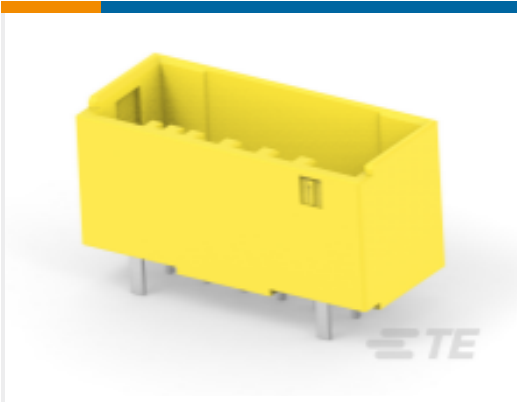
TE 产品编号1-2069574-6 DYNAMIC 1900D HDR ASSY V-TYPE 12P YELLOW
