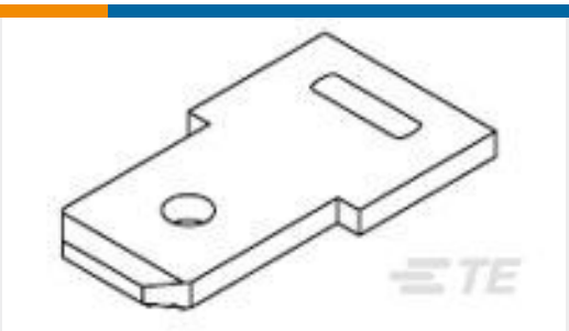
TE 产品编号42559-1 FASTON 250 SERIES (6.3 MM) TAB NPST
