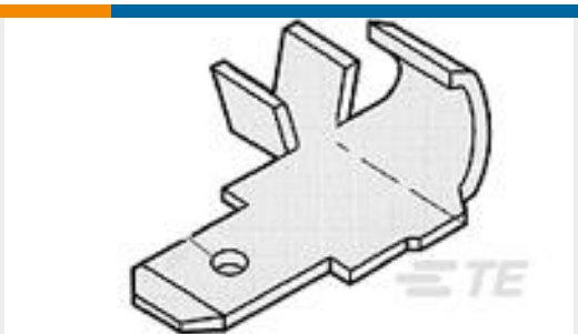
TE 产品编号42770-2 FASTON 250 FLAG TAB 18-14 TPBR
