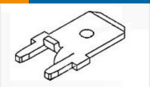
TE 产品编号1217126-1 250 FASTON,PCB TAB,TPBR
