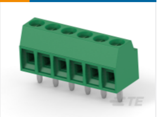
TE 产品编号1546551-6 6P,STRAIGHT,SIDE ENTRY,3.5MM
