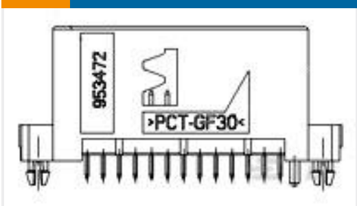
TE 产品编号953472-1 26pos MQS .63 header 180deg THR
