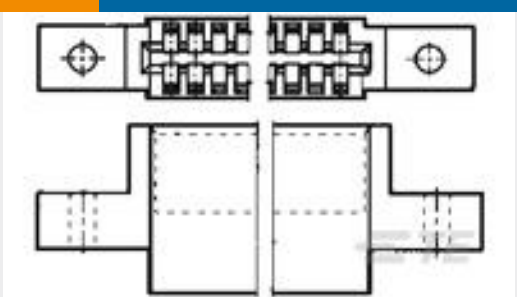
TE 产品编号1-583861-1 TW-LEAF CRP. HSG 17 POS. 100 C
