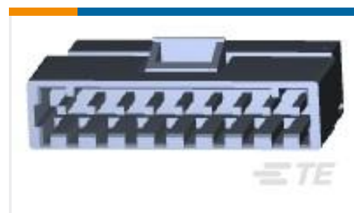
TE 产品编号647476-9 09P MTA156 PSTD CONN CE 18AWG
