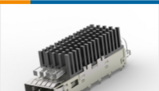
TE 产品编号2293574-1 CAGE ASSY, QSFP28 1X1, SPRING, HS, LP
