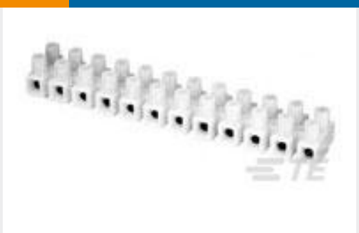
TE 产品编号1776296-3 TSB5000331DS=EUROPA T-BLK,10MM
