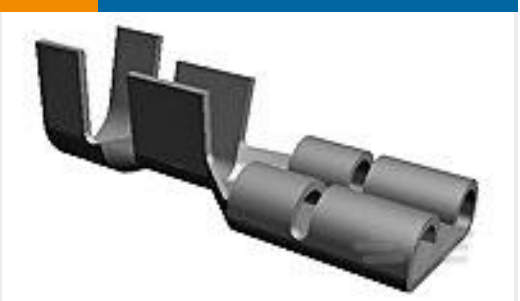
TE 产品编号100495-2 250 FASTON,LIF REC.,16-20 AWG, TPBR
