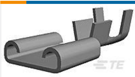
TE 产品编号170183-1 250 FASTON,REC.,22-18 AWG,BR
