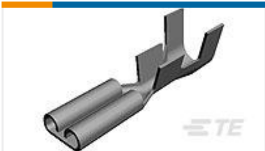
TE 产品编号170213-2 250 FASTON,REC.,18-14 AWG,TPBR
