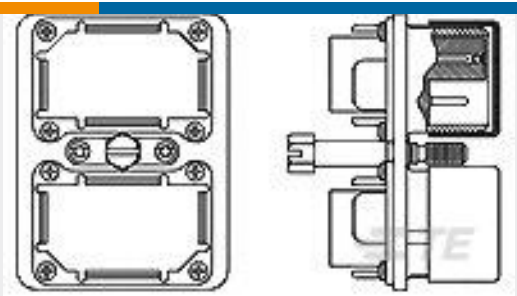
TE 产品编号213441-9 MME2P106S106S-0001 (204)
