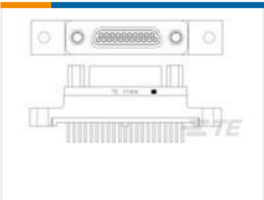
TE 产品编号 1532268-6 M83513/22-C02CP = MCKS-C2-P-21PST1A
