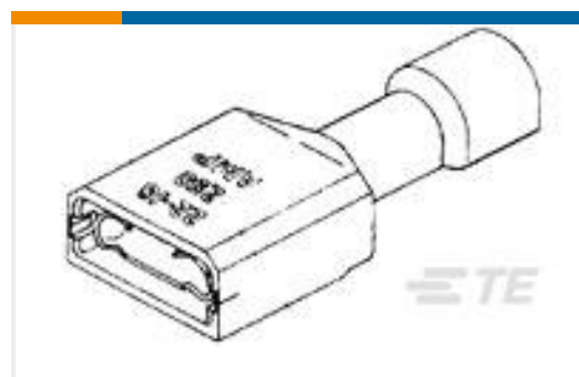
TE 产品编号2-520084-2 ULTRAFast 110 ASSY REC 22-18 TPBR LP
