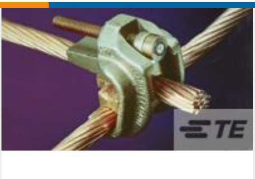
TE 产品编号83750-1 WRENCH-LOK 250-250
