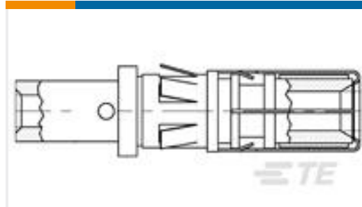
TE 产品编号202418-1 SKT CONT ASSY,TYPE I
