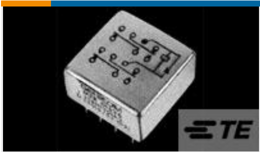
TE 产品编号 2-1617076-4 3SBH1227A2 = M39016/53-008M
