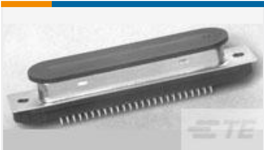
TE 产品编号553443-2 ASSY RCPT,ACTION PIN,CHAMP-LOK
