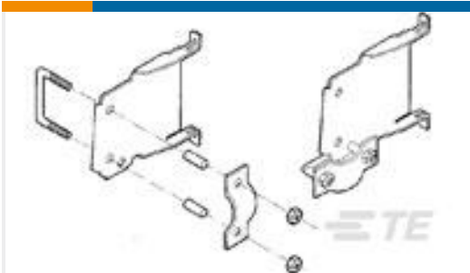
TE 产品编号201848-5 STRAIN RELIEF CLAMP UNASSEM.
