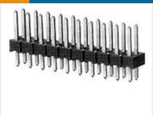
TE 产品编号3-102977-3 66 MODII HDR DRST B/A .100CL
