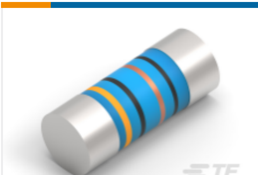
TE 产品编号2-2176316-6 MELF SMA_A 12K 0.1% 15PPM 0207 1W
