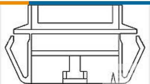
TE 产品编号1-103682-1 12 MTE PANEL MOUNT SR
