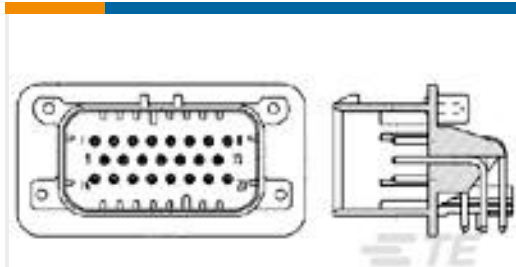
TE 产品编号1-776087-5 23 POS AMPSEAL HDR SNAP IN W/G
