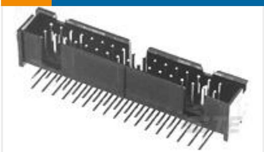
TE 产品编号5103311-8 A/L LOW PRO HDR 40P RA BLACK
