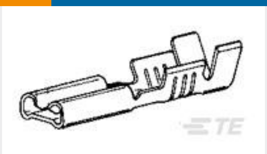
TE 产品编号160626-2 110 FASTON,REC.,20-17 AWG,TPBR
