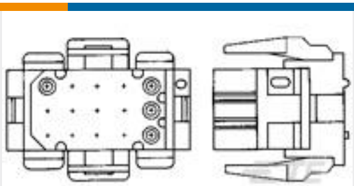
TE 产品编号1-640512-0 12P MR II CAP HSG V0 RED
