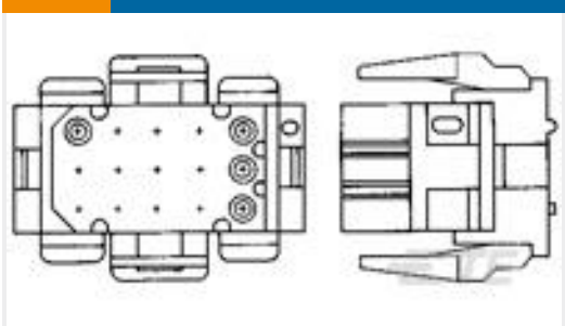
TE 产品编号1-640523-0 15P MR II PLUG HSG V0 RED
