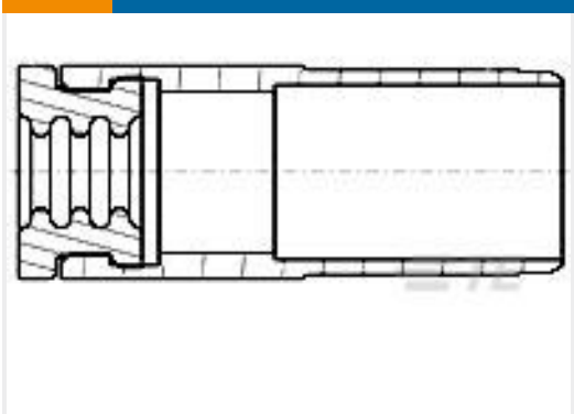
TE 产品编号1877626-1 Seal Assembly,Size 8 GPR
