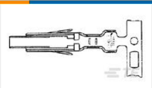
TE 产品编号170484-1 CONTACT FOR DRAWER CONNECTOR
