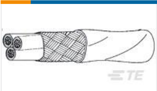
TE 产品编号306369-002 44AM1131-24-0/2/9-9
