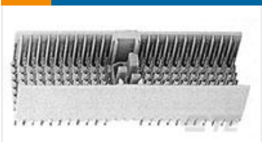
TE 产品编号188834-1 Z-PACK/A M-HDR 154P.
