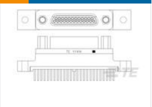
TE 产品编号1532269-1 M83513/22-D01CN = MCKS-C2-B- 25PST1
