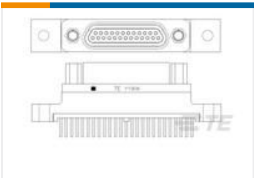
TE 产品编号1532277-1 M83513/25-D01CN = MCKS-C2-B- 25SST1
