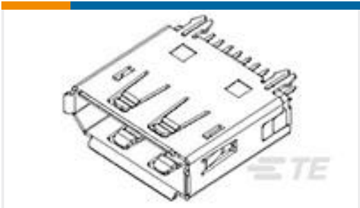
TE 产品编号2041441-3 Displayport,20P,Vertical,DIP Type,15u"
