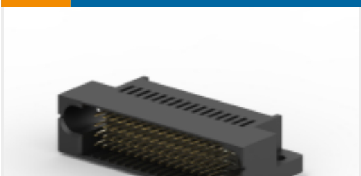
TE 产品编号1-6450520-3 MBXL R/A HEADER W/ GUIDE 64S
