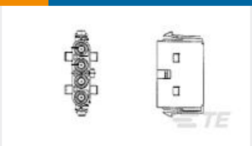
TE 产品编号794118-1 04P .156 MNL CAP PANEL MOUNT
