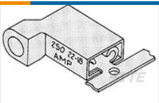
TE 产品编号2-520334-2 ULTRAFAST 187 ASSY FLAG REC 22-18 TPBR
