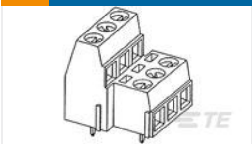
TE 产品编号1-796692-0 TERMI-BLOK PCB MOUNT 1&2 10P.5
