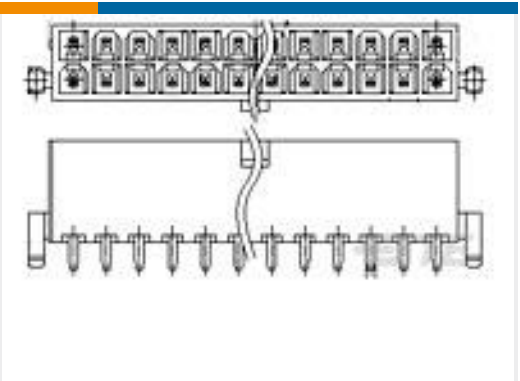
TE 产品编号2-1775099-0 ATX PWR CONN 2 BDLK 4 POS
