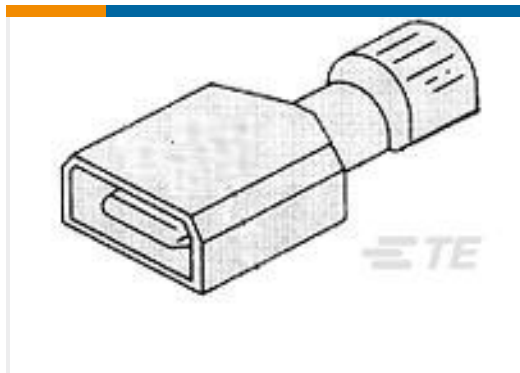
TE 产品编号3-520107-2 ULTRA-FAST 250 ASY TAB 16-14 AWG TPBR
