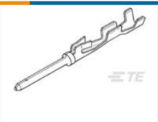
TE 产品编号1-745266-0 PIN CONTACT,HDE-20,#22-26 AWG
