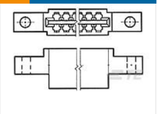
TE 产品编号583685-1 HSG AMP LEAF 30 POS
