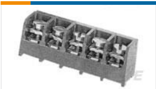
TE 产品编号2-1546158-3 6DBL-05-006=6DBL ASSEMBLY
