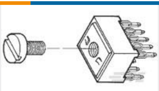
TE 产品编号 2307526-1 NECTOR M 7P SEALED SOCKET PCB CODE A
