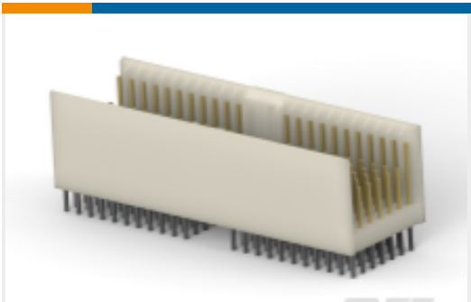
TE 产品编号3-100668-0 Z-PACK M.ASSY.154P.
