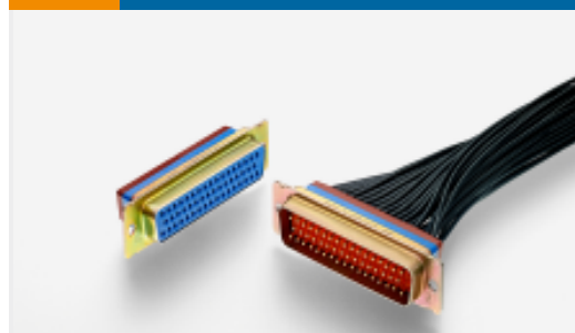
TE 产品编号1-2221760-6 AMPLIMITE IP67, SZ6, 90, 104 POS, RCPT
