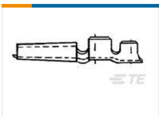
TE 产品编号41646 TAPER PIN, ON STRIP, GOLD; 53SER
