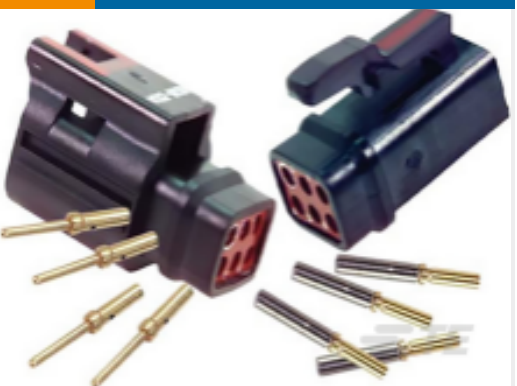
TE 产品编号ASC605-06PN PLUG.AS MODULAR.PIN.
