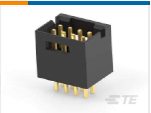
TE 产品编号3-87690-5 08 MODII HDR DRST SHRD .100CL
