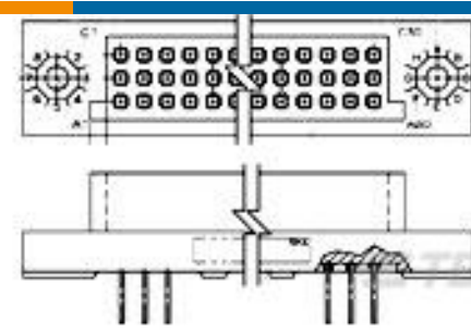
TE 产品编号531134-6 3ROW BOX REC 180P 100CL UNSEAL
