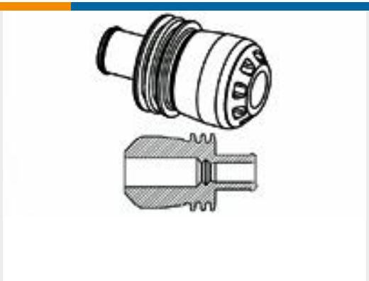
TE 产品编号1544664-1 WIRE SEAL 8NG1
